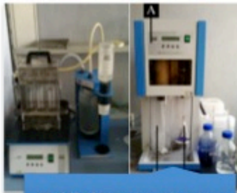
Kjeldhal Nitrogen digester with steam distillation unit
