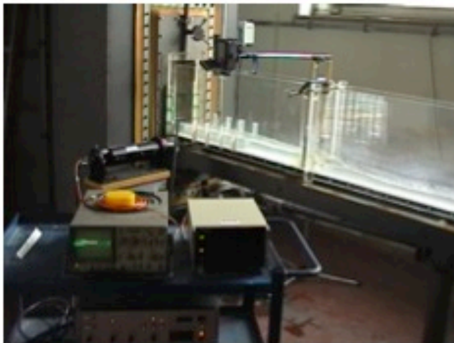
Physical model of a grass lined channel
